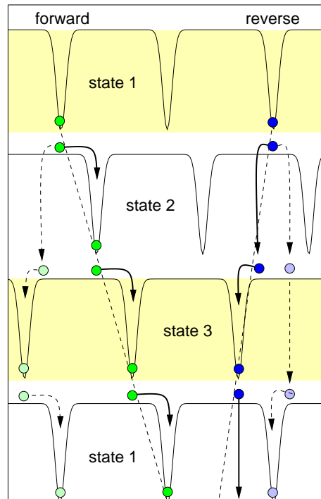
FIG. 1: A spatially-symmetric three-state ratchet potential comprised of discrete potential wells.
