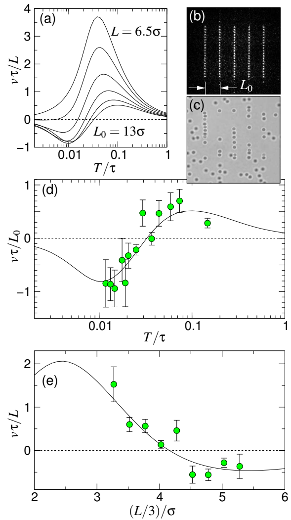
FIG. 2: (a) Crossover from deterministic optical peristalsis at L = 6.5\sigma to thermal ratchet behavior with flux reversal at L = 13\sigma for a three-state cycle of Gaussian well potentials at \beta V_0 = 8.5 , \sigma = 0.53\ \mu\text{m} and D = 0.33\ \mu\text{m}^2/\text{sec} . Intermediate curves are calculated for evenly spaced values of L . (b) Image of 20 \times 5 array of holographic optical traps at L_0 = 6.7\ \mu\text{m} . (c) Image of colloidal silica spheres 1.53\ \mu\text{m} in diameter interacting with the array. (d) Rate dependence of the induced drift velocity for fixed inter-trap separation, L_0 . (e) Separation dependence for fixed inter-state delay, T = 2\ \text{sec} .
